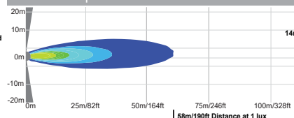
XIL-S1130 | 9888163 - 30° BEAM
