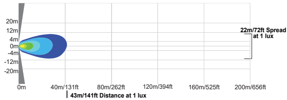
MAR-EPX760 | 9892115 - 60° Beam
