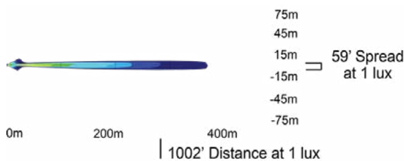
CTL-CPZ110WKIT | 9151069 - 10° Beam
