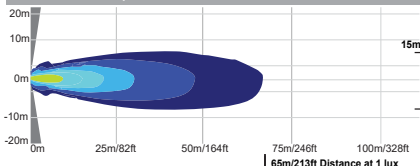
XIL-SP120 | 4009882 - 20° BEAM
