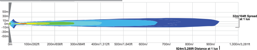
CTL-CPZ810 | 9890852 - 10° BEAM
