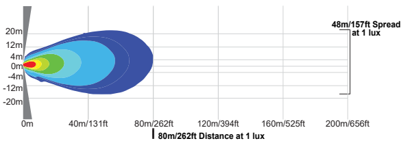
MIL-RXP1260T | 4009998 - 60° Beam
