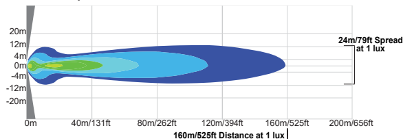
DURA-610 | 9891125 - 10° Beam
