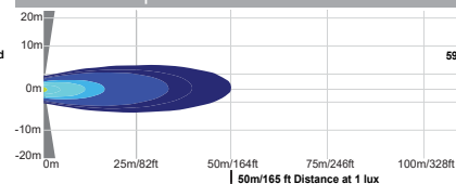
XIL-MX140 | 9113715 - 40° BEAM
