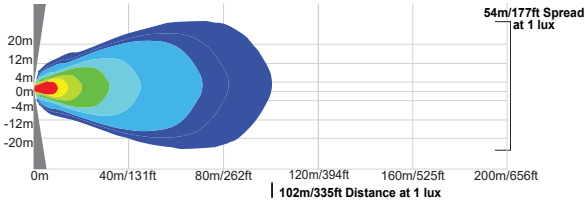
MIL-RXP2060T | 9114439 - 60° Beam
