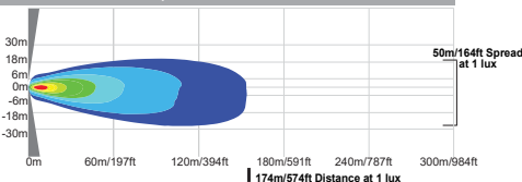
CTL-TPX1840 | 9111193 - 40° BEAM
