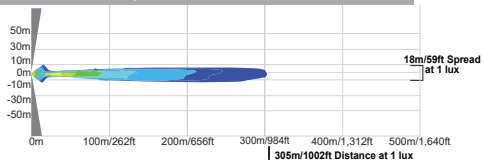
CTL-CPZ110 | 9150970 - 10° BEAM
