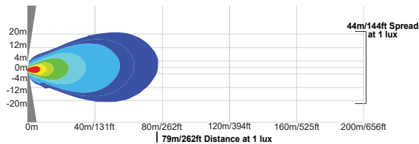
MAR-RXP1260 | 9892092 - 60° Beam
