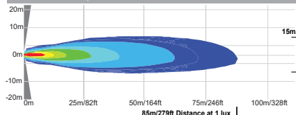
XIL-SP110 | 4008830 - 10° BEAM
