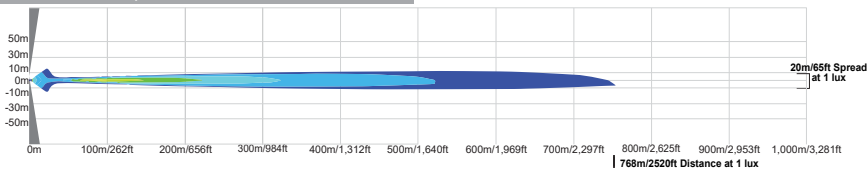
CTL-CPZ610 | 9888538 - 10° BEAM
