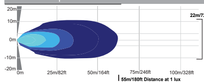
XIL-S1160 | 9888170 - 60° BEAM
