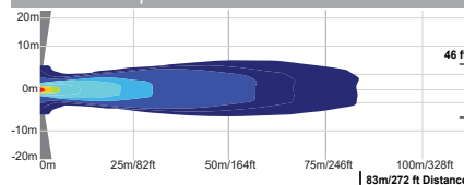
XIL-MX110 | 9113531 - 10° BEAM
