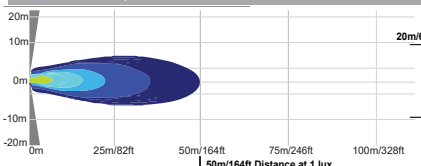
XIL-SP140 | 4009899 - 40° BEAM
