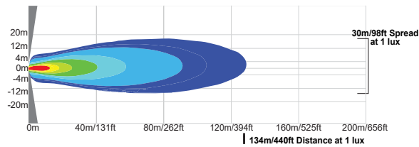
XIL-SP740 | 4009875 - 40° Beam
