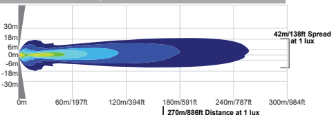
CTL-TPX1810 | 9111018 - 10° BEAM
