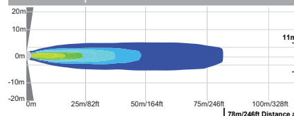
XIL-S1110 | 9888156 - 10° BEAM
