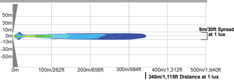
CTL-CPZ110XP | 9893259 - 10° BEAM
