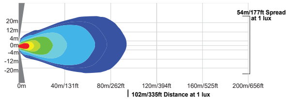
MAR-RXP2060 | 9892108 - 60° Beam
