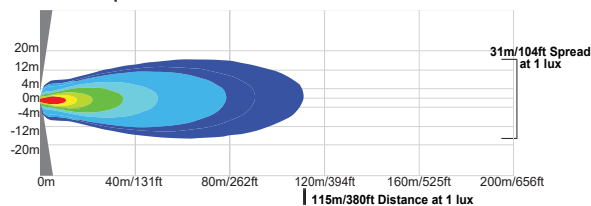
XIL-SP540 | 4009851 - 40° Beam
